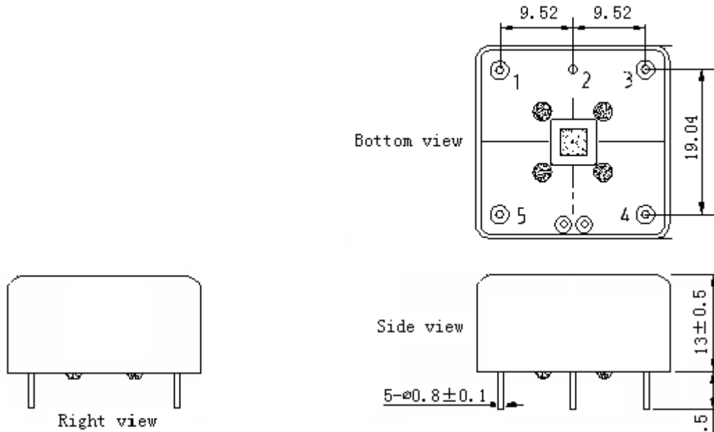
PIN FUNCTION
