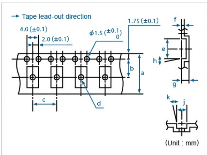
Conforming to JIS C 0806 TB1208NEIAJ and RC-1009B TE1208N
