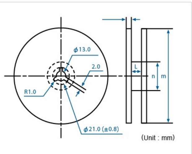
Conforming to JIS C 0806 R12R and EIAJ RC-1009B R15
