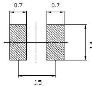
LAND PATTERN(REFERENCE)
