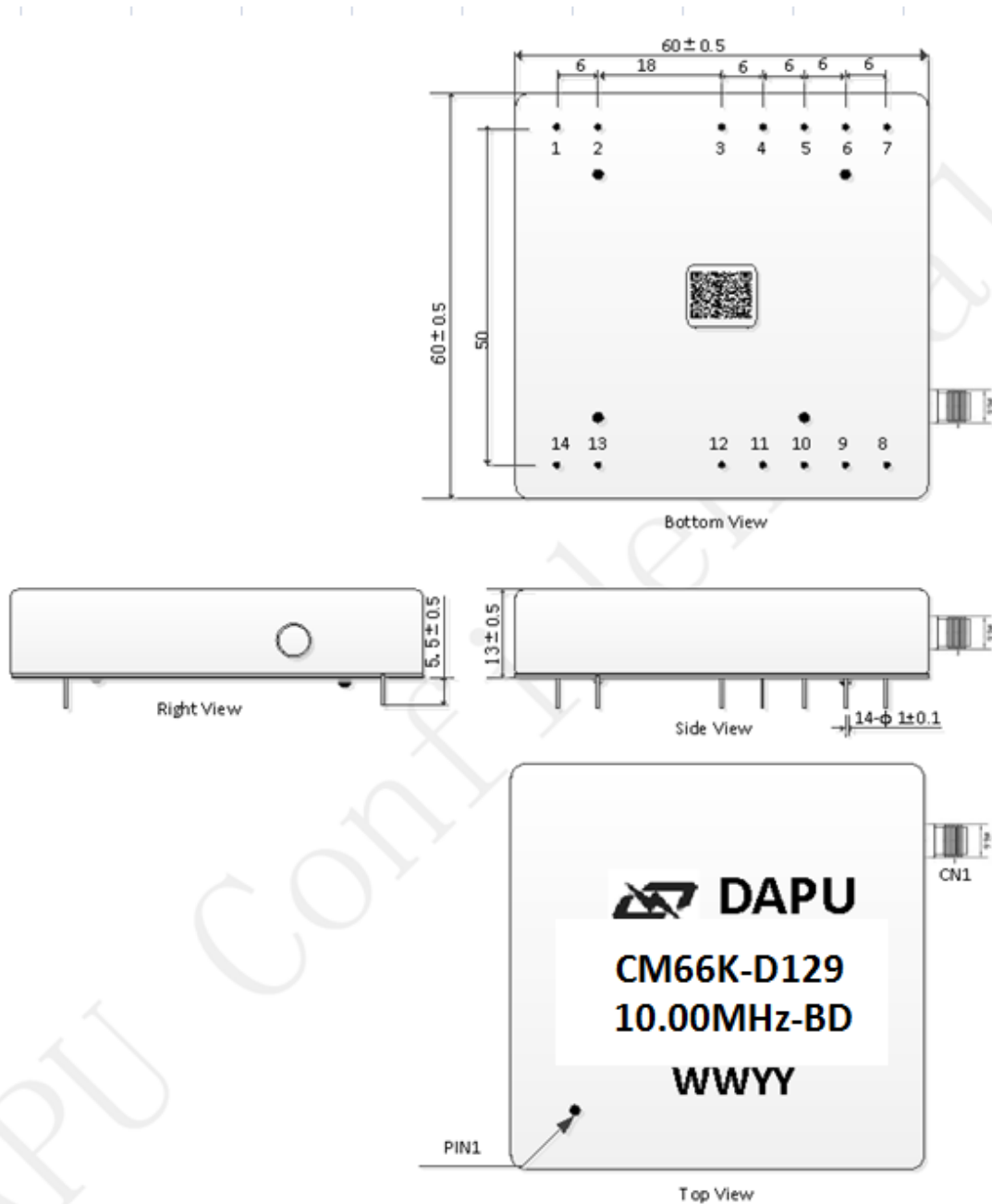
Figure 3 Mechanical structure
