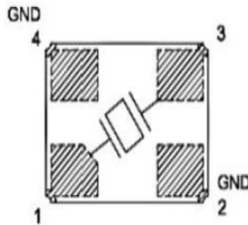
Internal Connections(Top View)
