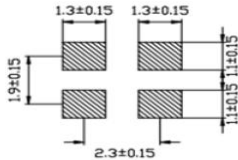
LAND PATTERN(REFERENCE)
