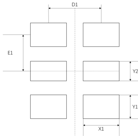
Figure 7.3. DSO3001 (5032 and 3225) PCB Land Pattern
