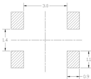
Solder pad layout
