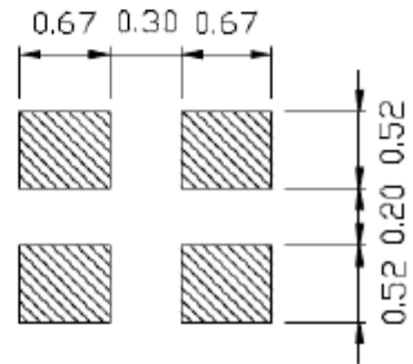
LAND PATTERN<REFERENCE>
