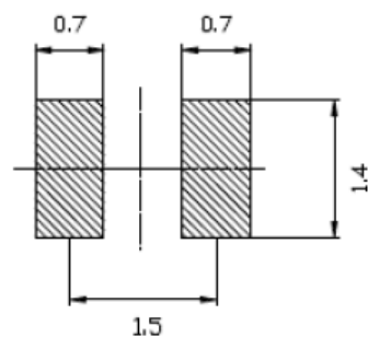
LAND PATTERN<REFERENCE>
