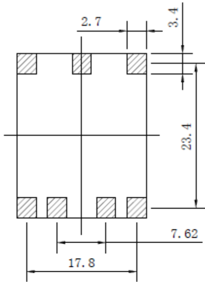
Solder Pad layout
