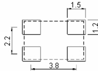
Recommend Soldering Pattern
