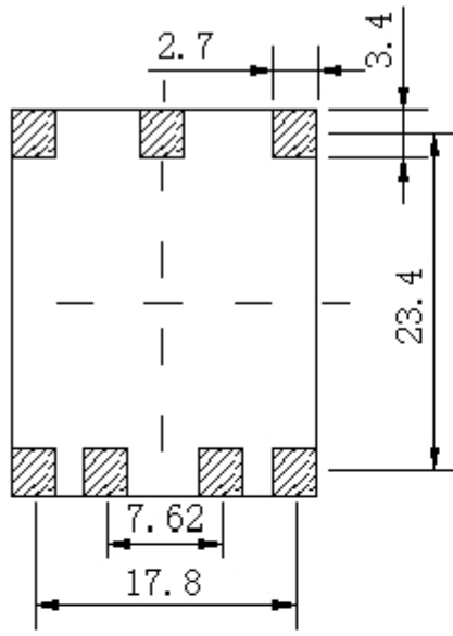
Solder Pad layout
