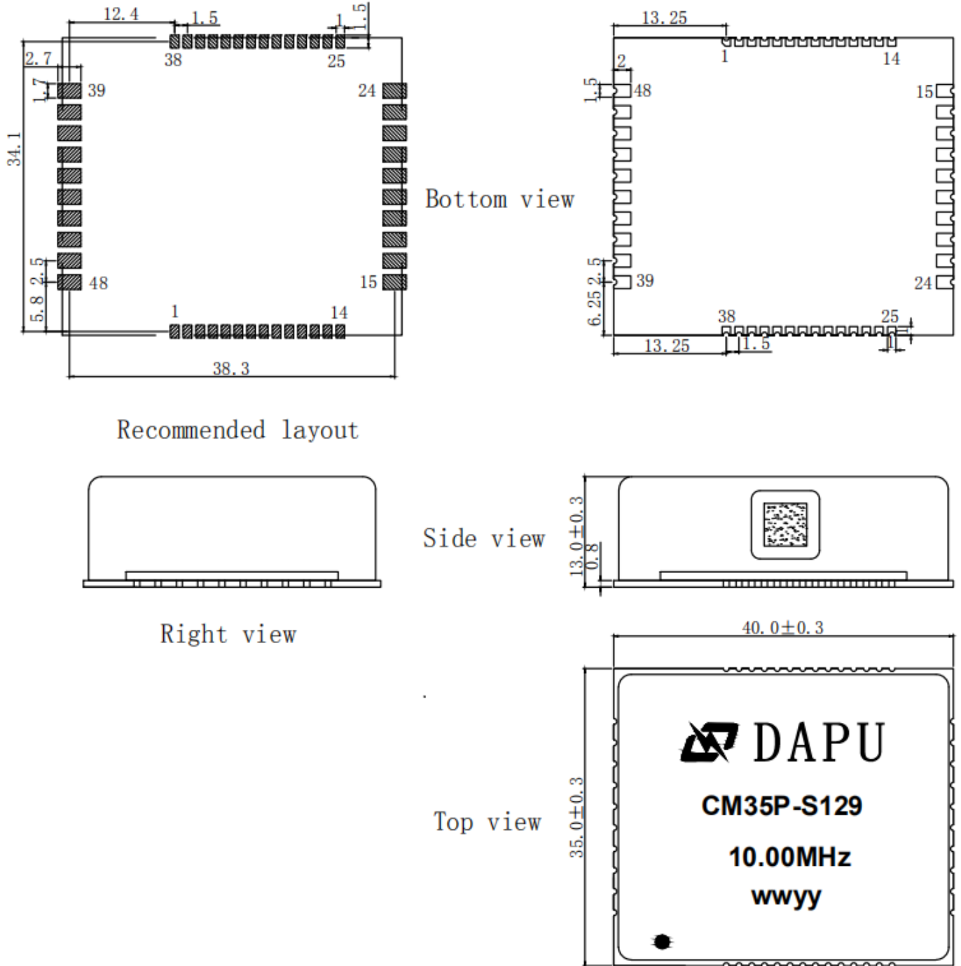
Figure 4 - Mechanical structure
