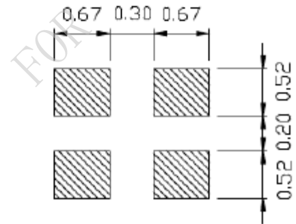
LAND PATTERN(REFERENCE)
