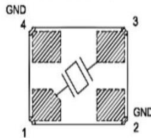
Internal Connections(Top View)
