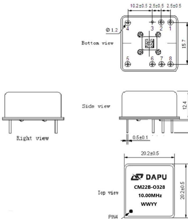
Figure 3 Mechanical structure
