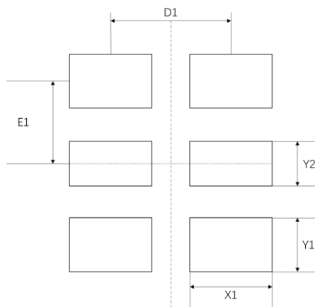
Figure 7.3. PCB Land Pattern
