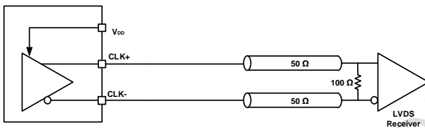
DC-Coupled LVDS
