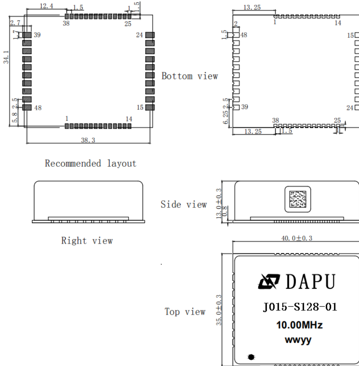
Figure 4 - Mechanical structure
