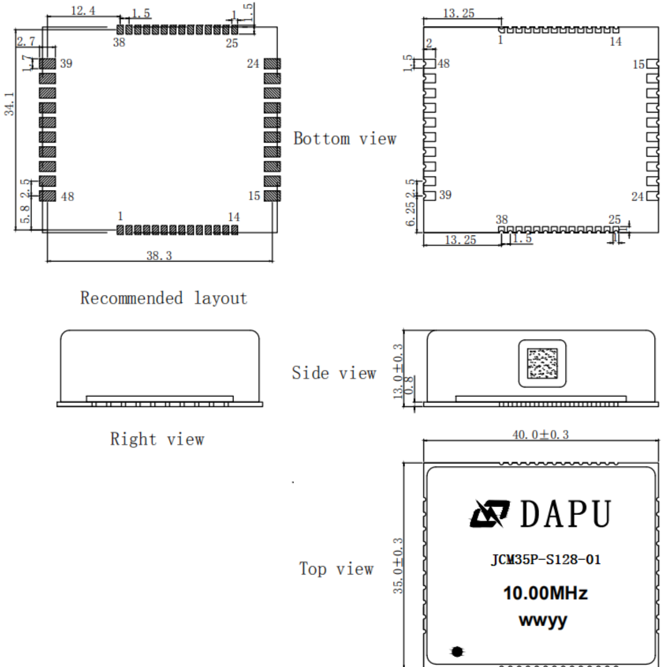
Figure 4 - Mechanical structure
