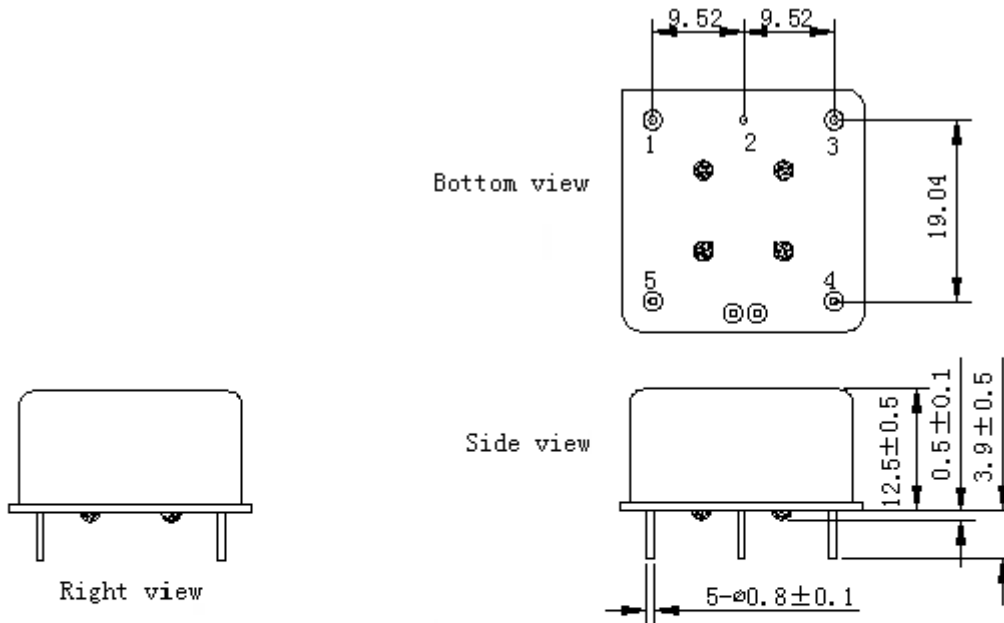
PIN FUNCTION
