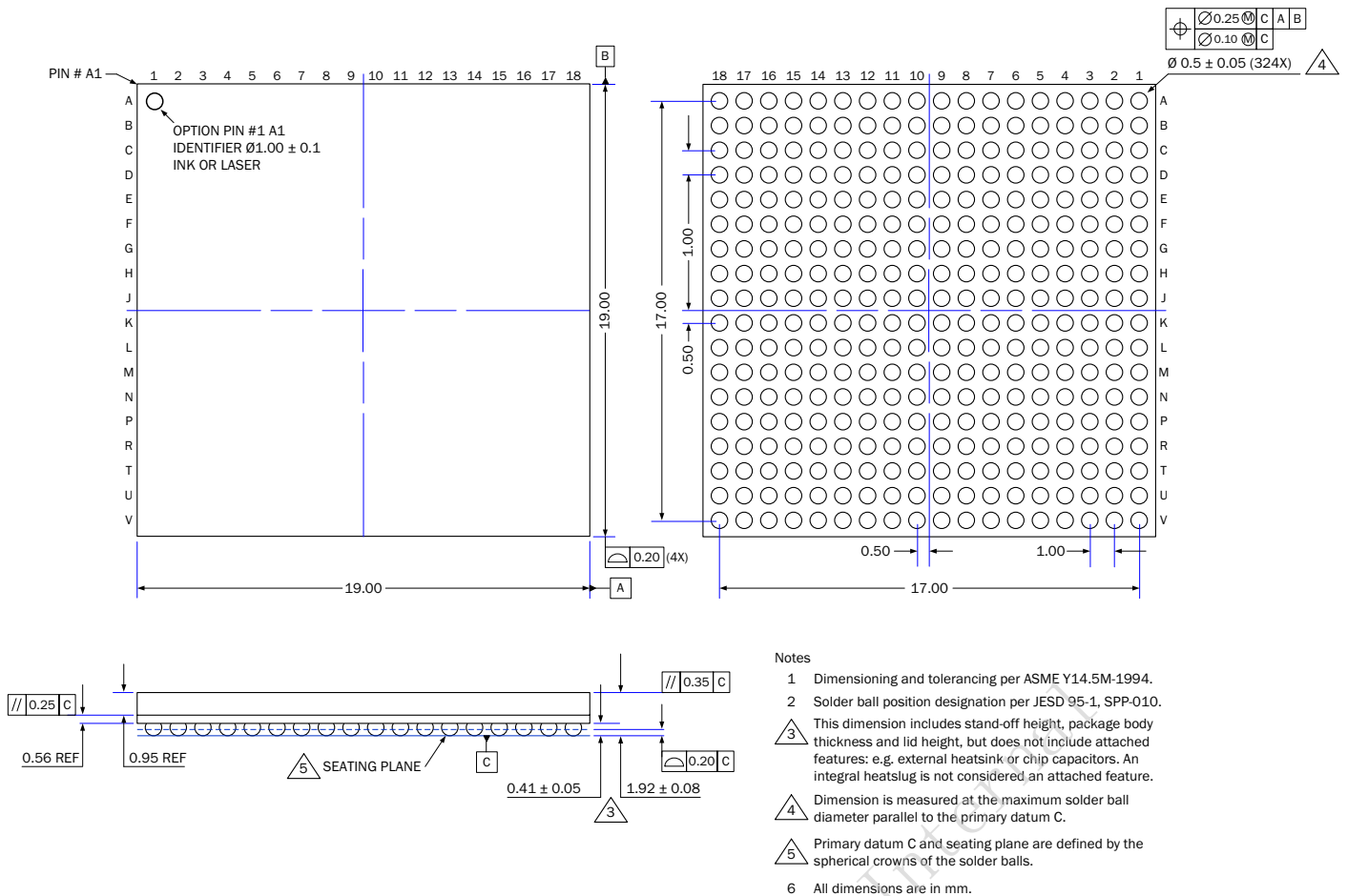
Figure 41 - LBG4 package, 1.0 mm pitch, 19 mm x 19 mm x 1.92 mm, 324 balls
