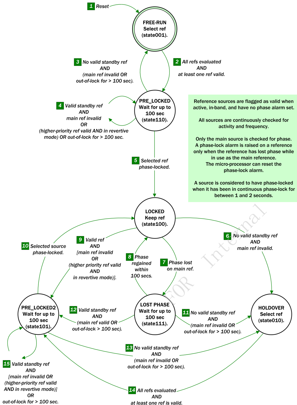
Figure 22 - Automatic mode control state diagram (T0 DPLL)
