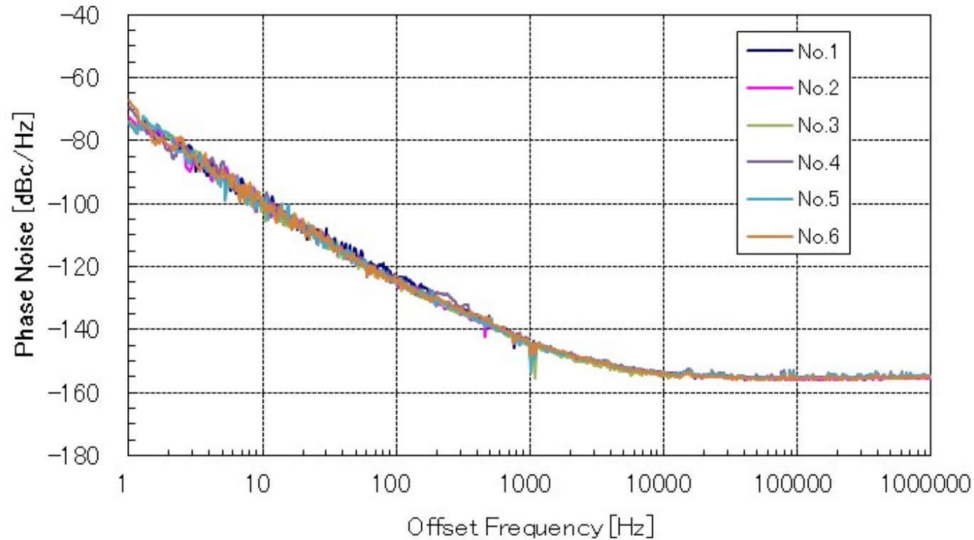
Fig1. Sample data of SSB Phase Noise (Frequency: 10.00MHz)
