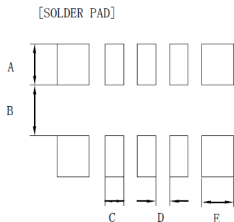
Figure 4. Dimensions and Recommended Solder Pad
