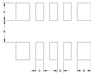
Figure 6. Recommended Soldering Pattern
