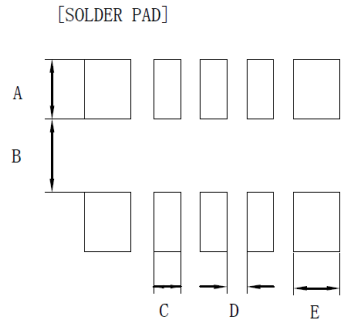
Figure 4. Dimensions and Recommended Solder Pad
