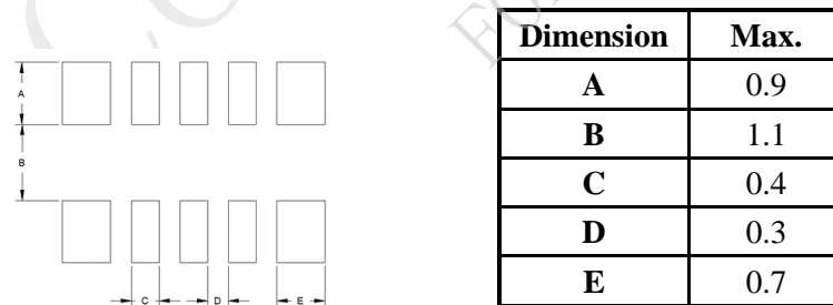
Figure 2. Recommended Soldering Pattern
