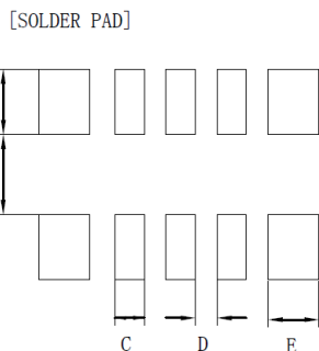
Figure 4. Dimensions and Recommended Solder Pad
